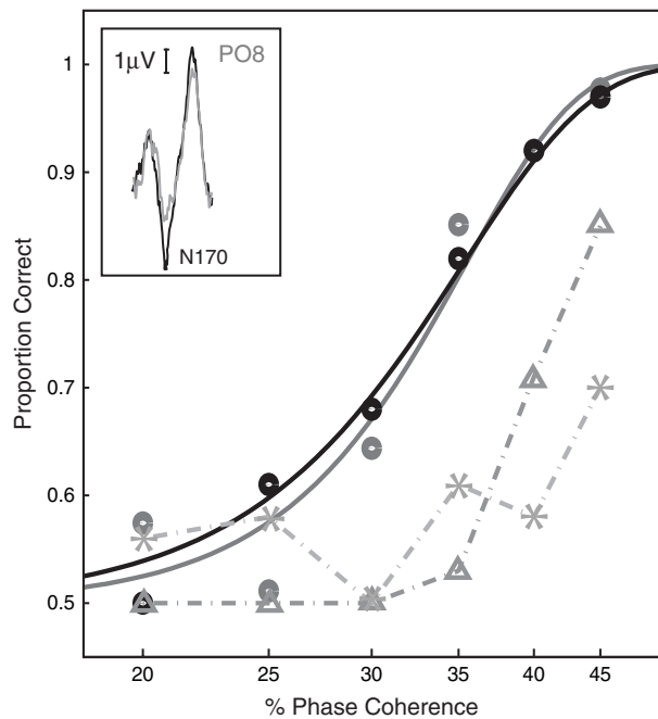
Figure 6. Comparison of a psychometric function (gray, solid circles) with neuro-metric functions constructed in three different ways: (i) the actual neuro-metric function (black, solid circles) constructed using our spatial integration algorithm (which weights all electrodes) and after integrating data from both the early and late windows. (ii) A neuro-metric function (gray triangles) constructed across both the early and late windows but for only a single electrode. We used electrode PO8 for single-electrode discrimination, because it showed the most significant difference between face (black) and car (gray) trials as indicated by the average ERP (see inset). (iii) A neuro-metric function (gray asterisks) constructed using the spatial integration algorithm (all electrodes) during a time window around this subject's median response time.
